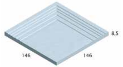
RSTC Askelmakulma, RT-pinta 66 + väri + RSTC
